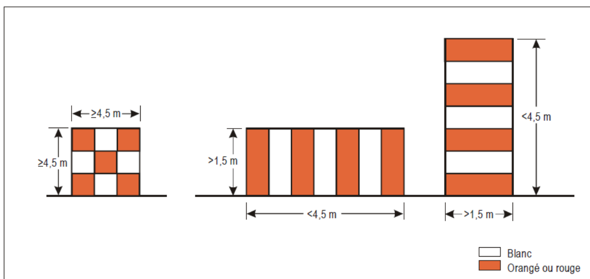
Figure 6-1. Marquages types
